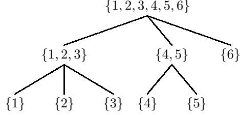
Figure 2.2: A dimension partition tree related to \mathbf{V}_D = \mathbf{V}_{123} \otimes_a \mathbf{V}_{45} \otimes_a V_6 .
